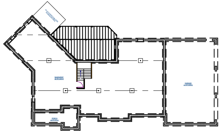
FOUNDATION PLAN
