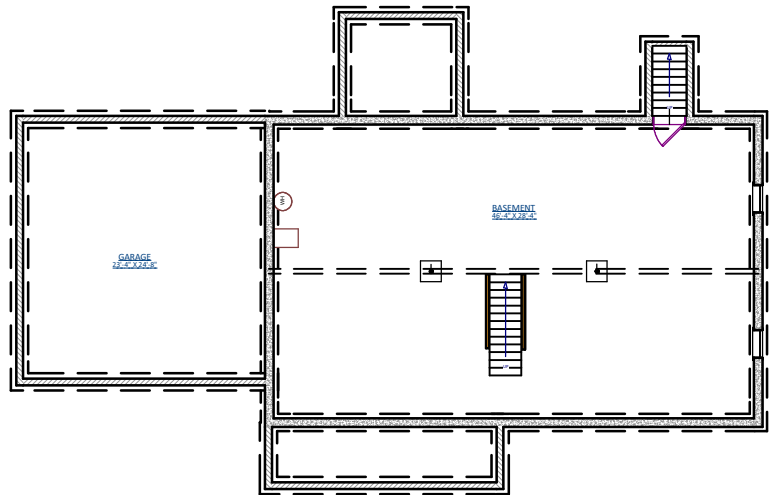
FOUNDATION PLAN
